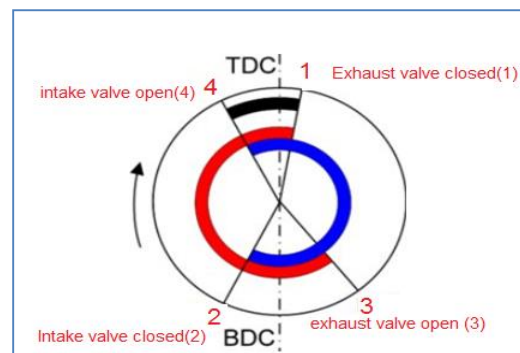
Figure 2: Valve timing diagram [29]
