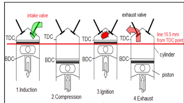
Figure 1: 4- stroke engine stages with valves and the 15.5mm line location
