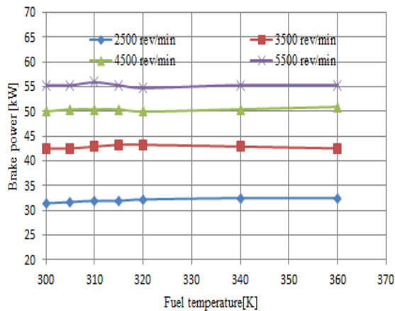
Figure 11: brake power of the engine at different fuel temperature and engine speed
