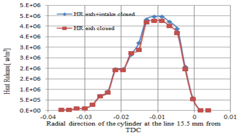
Figure 5: heat release at the line 15.5 mm below TDC point
