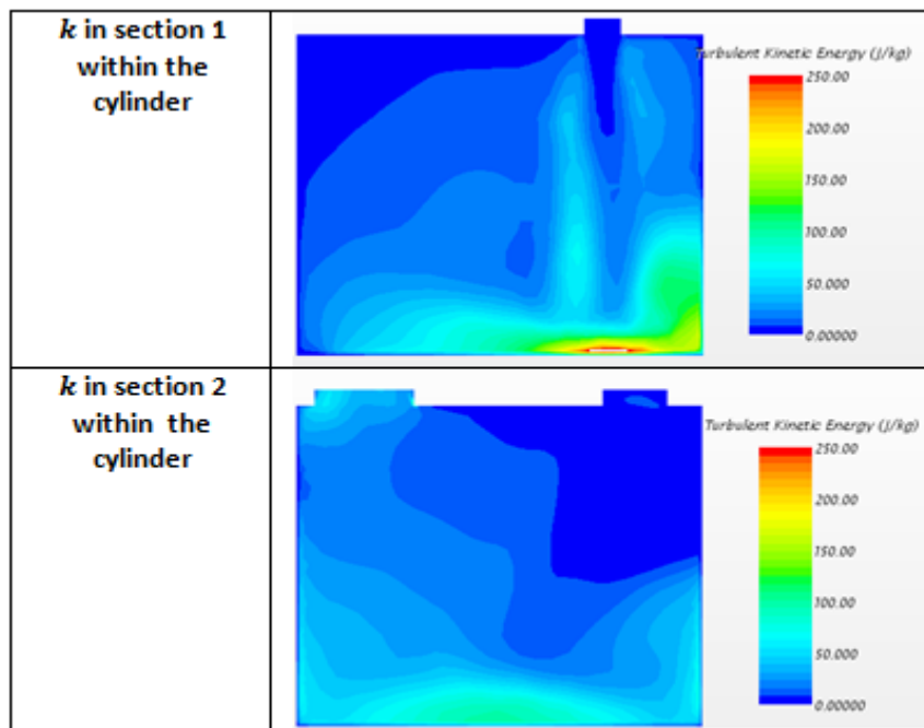
Figure 8: Turbulent kinetic energy k contour in sections 1 and 2 in the cylinder at exhaust valve open
