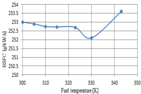
Figure 12: the brake mean specific fuel consumption in different fuel temperature at engine speed 2500 [rev/min]
