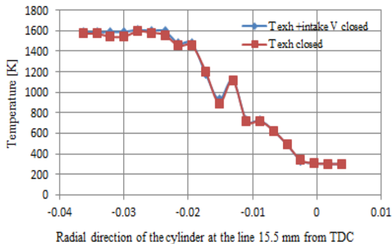
Figure 6: temperature distribution at the line 15.5 mm below TDC point
