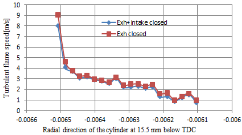
Figure 4: turbulent flame speed S_T distribution at the line 15.5 mm below TDC
