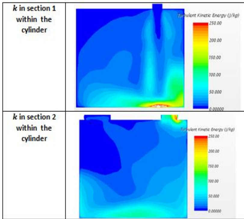
Figure 7: Turbulent kinetic energy ( k ) contour in sections 1 and 2 in the cylinder at exhaust valve closed
