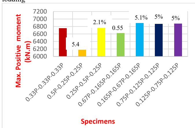
Figure 15. Group C: load-carrying capacity under unbalanced loading
