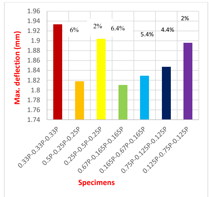
Figure 12. Group B: peak deflection under unbalanced loading
