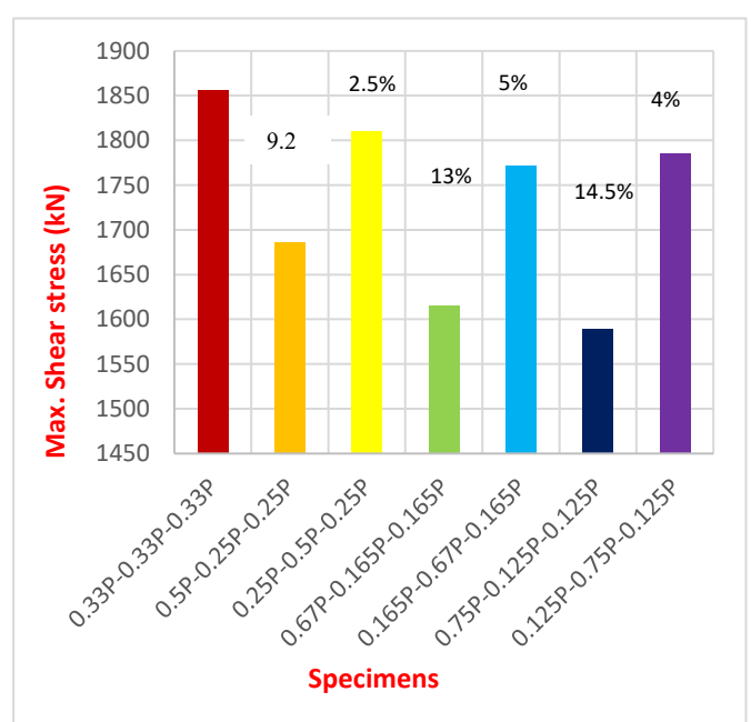
Figure 10. Group A: peak shear stress under unbalanced loading
