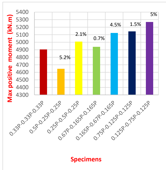
Figure 9. Group A: peak bending moment under unbalanced loading
