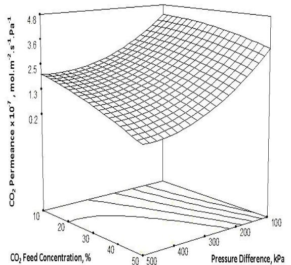
Figure 2: Effect of pressure difference across the HT-silica membrane and CO 2 feed concentration on CO 2 permeance at temperature of 110 °C
