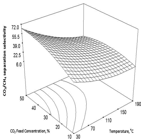
Figure 6: Effect of temperature and CO 2 feed concentration on CO 2 /CH 4 separation selectivity at pressure difference across the HT-silica membrane of 300 kPa
