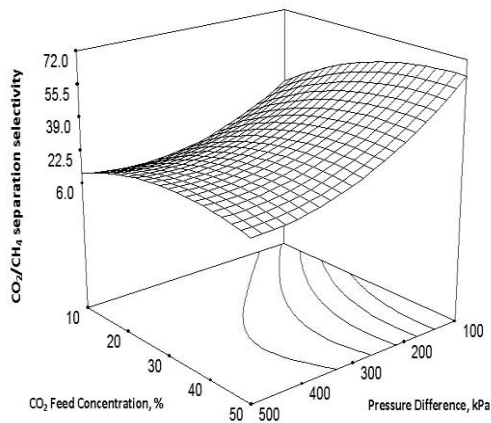
Figure 5: Effect of pressure difference across the HT silica membrane and CO 2 feed concentration on CO 2 /CH 4 separation selectivity at temperature of 110 °C
