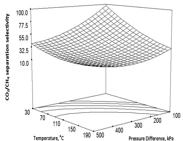
Figure 4: Effect of pressure difference across the HT-silica membrane and temperature on CO 2 /CH 4 separation selectivity at 30% CO 2 feed concentration
