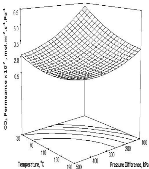
Figure 1: Effect of pressure difference across the HT-silica membrane and temperature on CO 2 permeance at 30% CO 2 feed concentration
