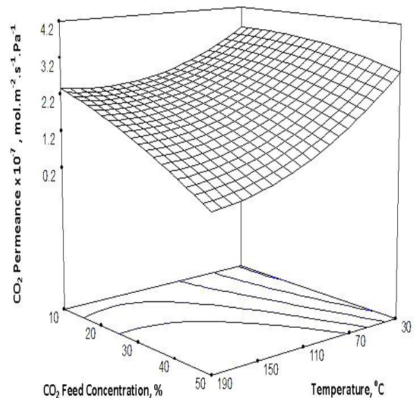
Figure 3: Effect of temperature and CO 2 feed concentration on CO 2 permeance at pressure difference across the HT-silica membrane of 300 kPa
