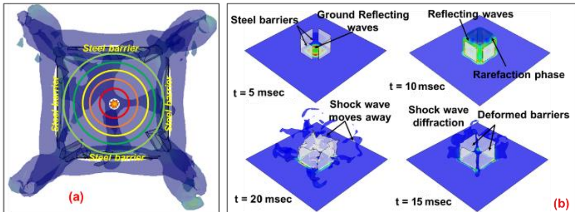
Figure 7. Blast shock wave phenomena of suicide vest burst a. top view b. 3-D view of suicide vest blast wave environment
