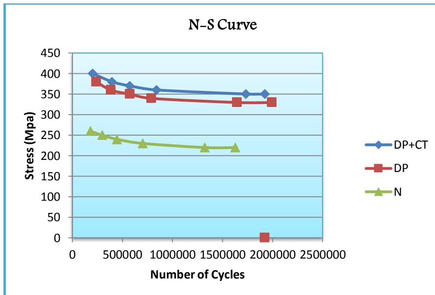
Fig.4 fatigue limits before and after cryogenic treatment
