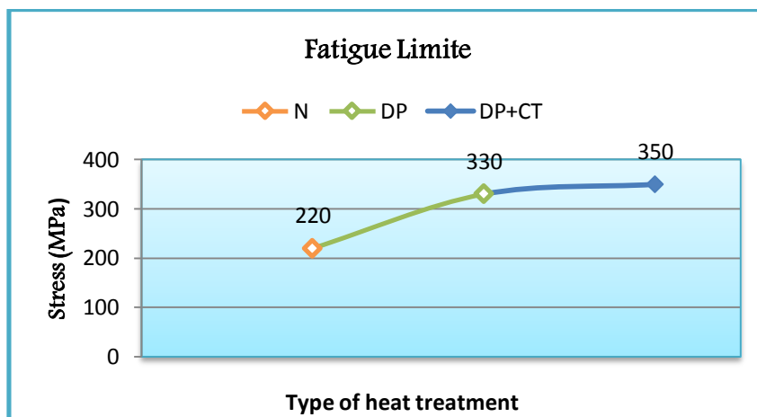
Fig.5 shows enhancement of endurance limit according with type of heat treatment
