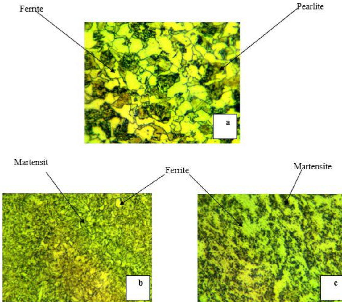
Figure7 shows the microstructure of a -normalized steel b -ferritic-martensitic steel before c -after cryogenic treatment.
