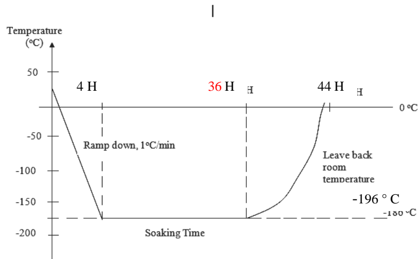
Fig.3 a typical cryogenic treatment for 17Mn4 steels.
