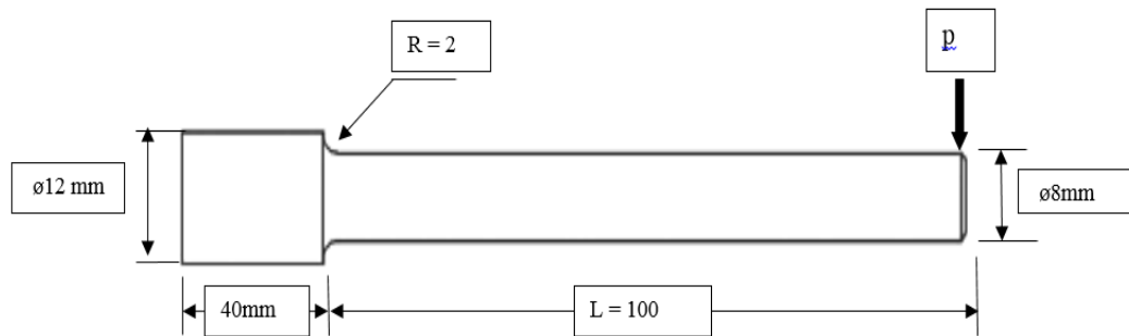
Fig.2 Fatigue test sample dimensions
