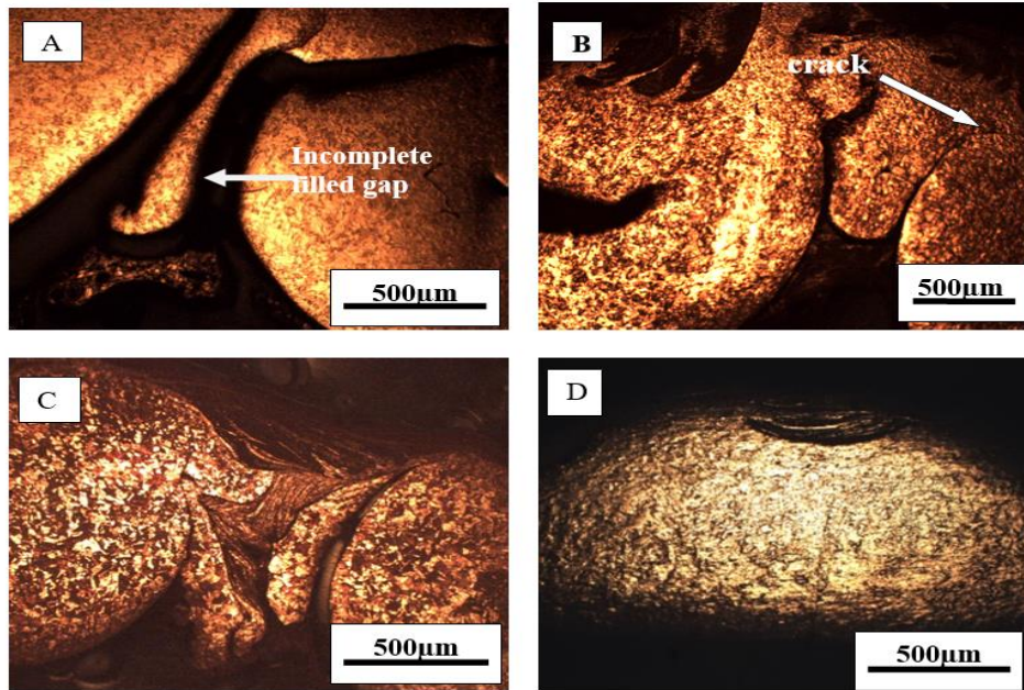
Fig. 6. Microstructure of FCWed Cu-Cu joints at different tool rotational speeds and feed rates (A) 220 rpm tool rotational speed and 20 mm/min feed rate, (B) 410 rpm tool rotational speed and 43 mm/min feed rate, (C) 920 rpm tool rotational speed and 80 mm/min feed rate, (D) 1500 rpm tool rotational speed and 115 mm/min feed rate
