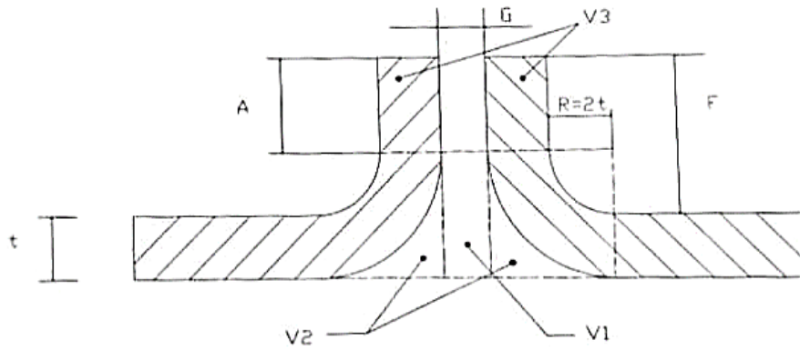
Fig. 3. Sketch of joint design of friction crush welding
