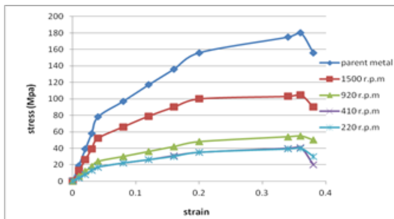
Fig. 9. Stress-strain curves of parent metal and FCWed Cu-Cu joints
