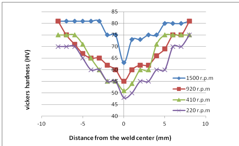
Fig. 7. The hardness distribution along a cross section of FCWed copper joint at various tool rotational speeds
