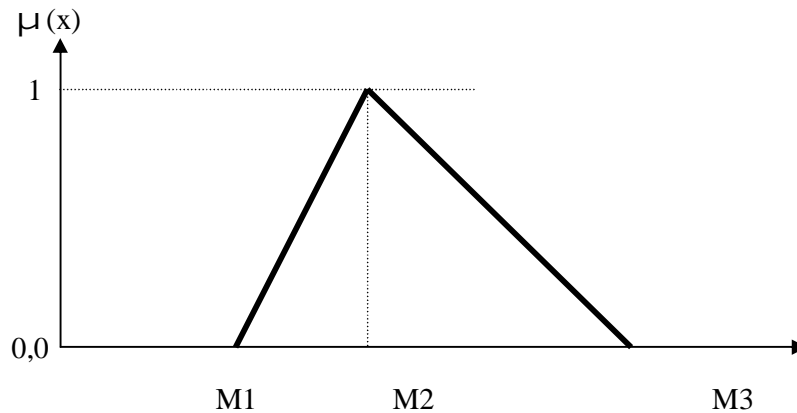
Fig.(1): Fuzzy Triangular Number representation (7) .
