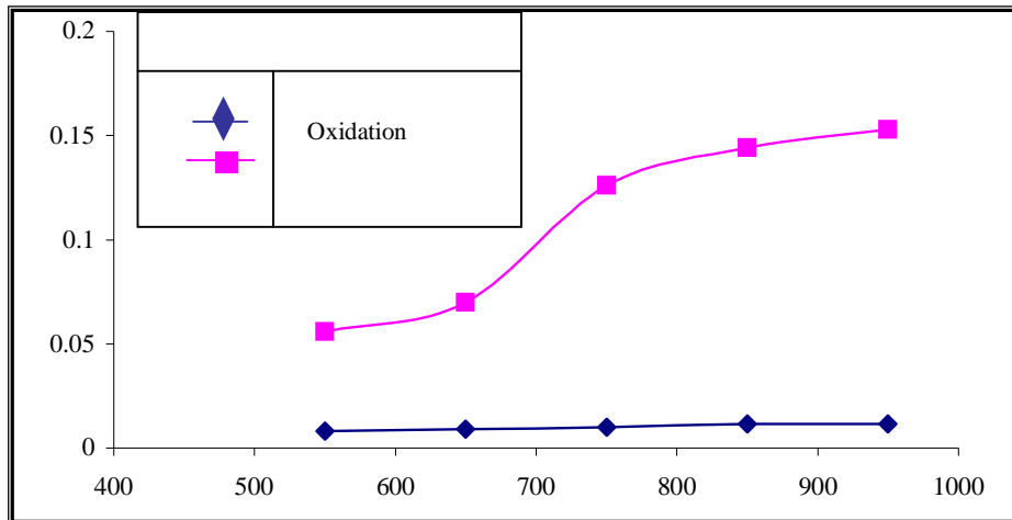
Fig.(2): Effect of heating Temperature and Weight Gain for 209 T1 Specimens at four hours of exposure.
