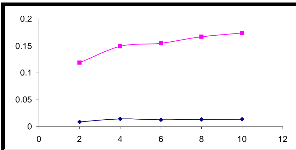
Fig.(4): Effect of exposure Time on Weight Gain for (213 T11) Specimens at 950 °C.
