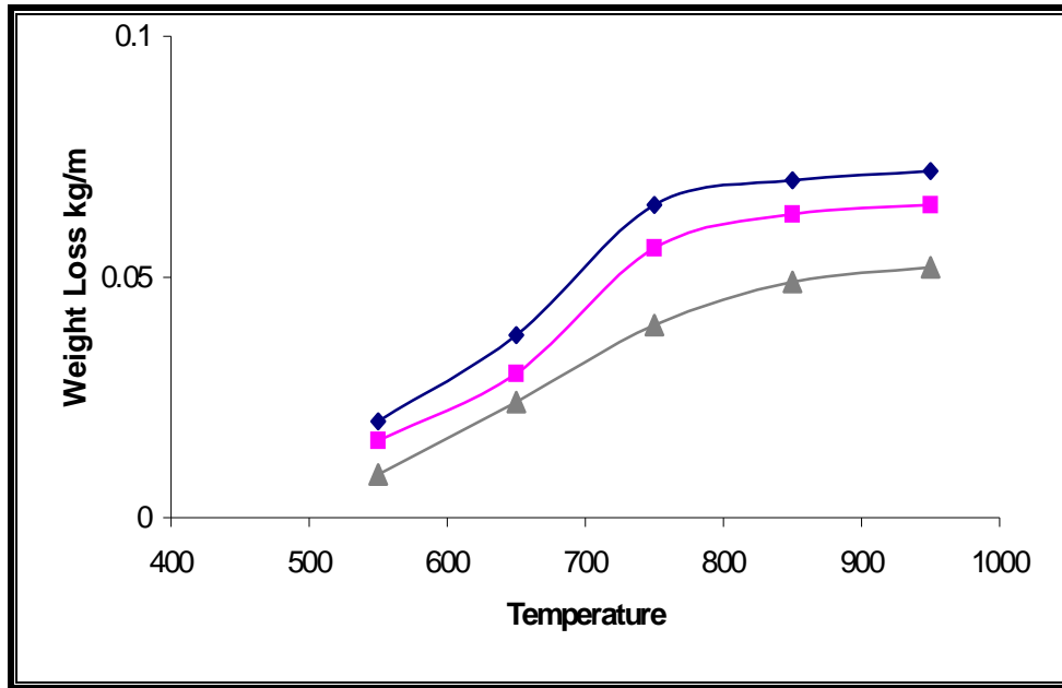
Fig. (5): Effect of Temperature on weight loss at various Ratios of Mg(OH)_2 :Ash for SA-178A Specimens at 4h.
