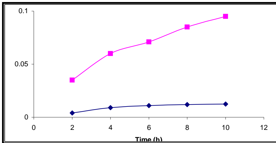
Fig. (3): Effect of exposure Time on Weight Gain for SA-178A Specimens at 550°C.
