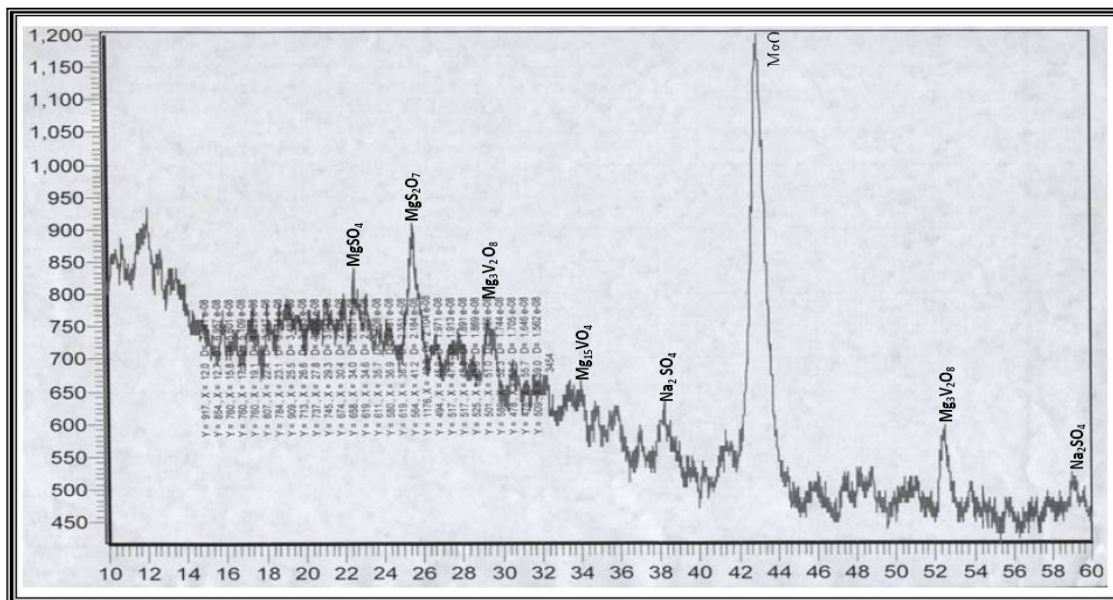
Fig.(8): X-ray Diffraction Pattern of Deposits on 213 T11 Specimen Coated with [3:1] Mg(OH) 2 :Ash, Heated at 750°C for 4h.
