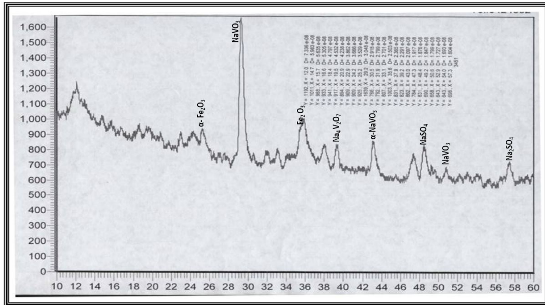
Fig. (7): X-ray Diffraction Analysis of Deposits on SA-178 Specimen Coated with Ash , Heated at 750°C and 4h.
