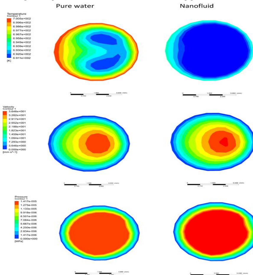
Fig 4. Temperature distribution versus surface outlet pipe at Re = 200
