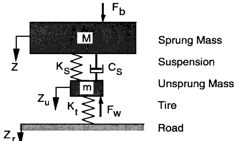
Figure 2. Mathematical model quarter car
