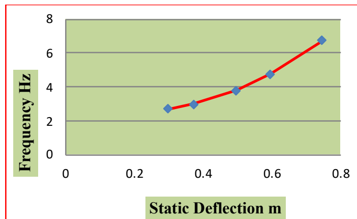
Figure 4. Relation between natural frequency and \delta .
