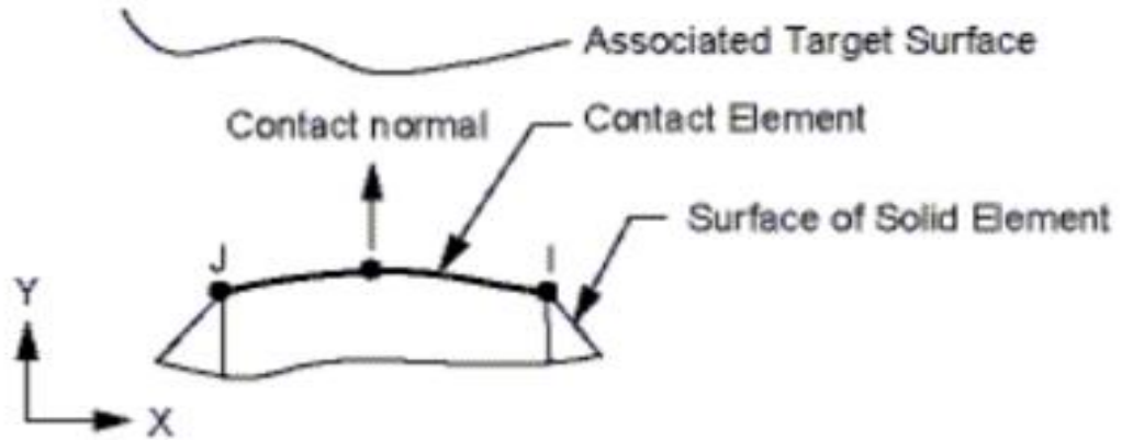
Figure 4. CONTA172 element geometry [8]
