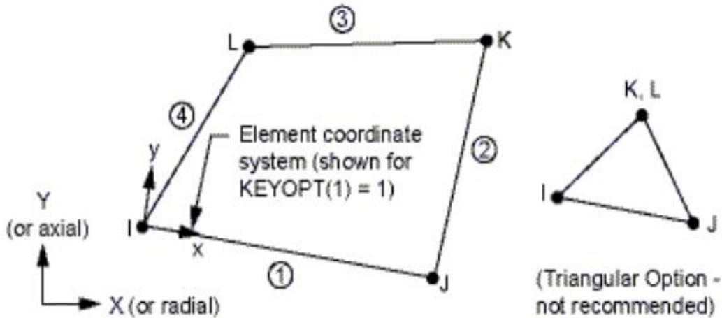
Figure 3. PLANE42 element geometry [8]
