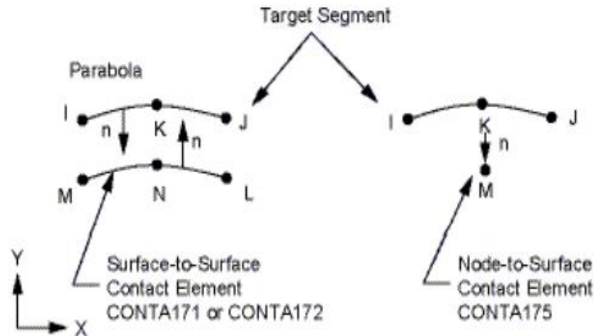
Figure 5. TARGE169 Element Geometry [8]
